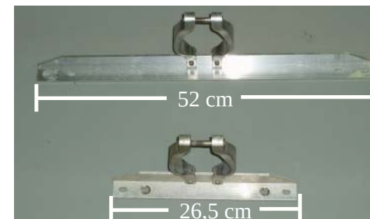
AF-Merkjafestingar 75mm.
