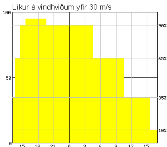
Figure 4. An example of a wind gust forecast for wind gusts > 30 m/s or higher for the meteorological station Hafnarfjall. This forecast is run on the 06 UTC analysis and published at 11 UTC on 07. Nov. 2011
